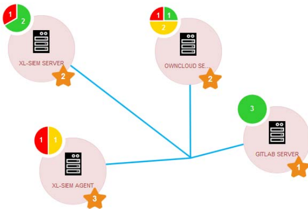
Fig. 2: Platform's Dashboard
